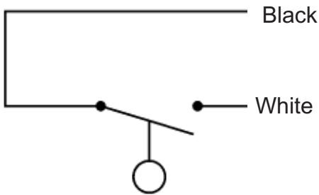
Fig. 1a - Normally Open
