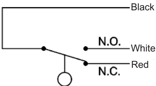
Figure 2 SPDT wiring diagram Dry Condition
