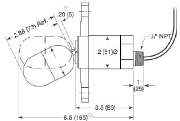
L070 with flanged connection and SPST or SPDT switch with flying leads
