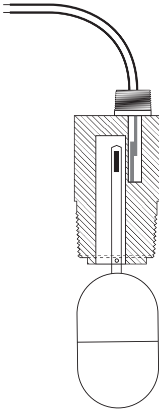
Figure 5 Cross section
