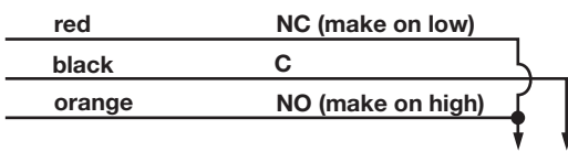
Figure 4 SPDT Flying leads wiring diagram
