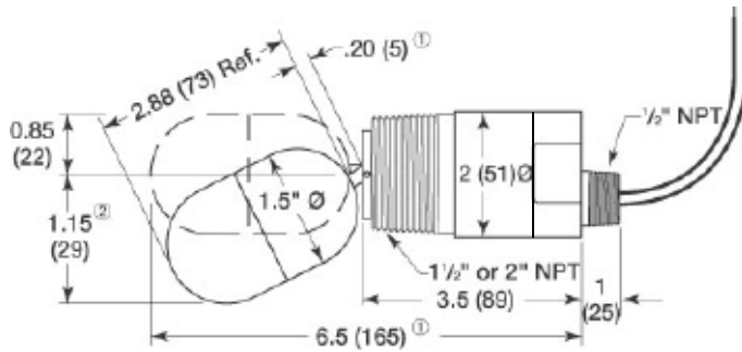
L070 with threaded connection and SPST or SPDT switch with flying leads
