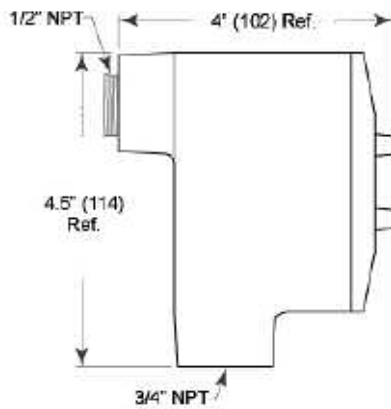
Junction box supplied with DPDT relay
