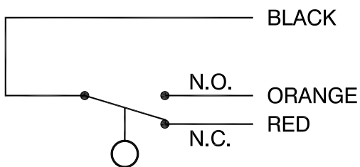
Figure 2 SPDT wiring diagram Dry Condition
