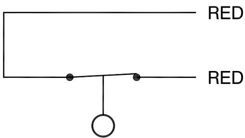
Fig.1b - Normally Closed
