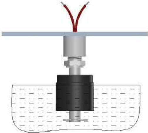
Top Mounting
